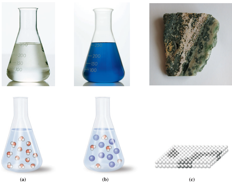
Figure 1.4 Schematic representations of some classes of matter. (a) A pure substance, water, consists of a single component. (b) A homogeneous mixture, blue dye in water, has a uniform distribution of components. The blue spheres represent the blue dye molecules. (c) The mineral orbicular jasper is an example of a heterogeneous mixture. The lack of homogeneity is apparent from its nonuniform distribution of components.
