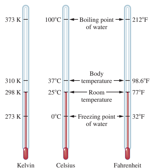
Figure 1.11 The freezing point and boiling point of water, body temperature, and room temperature expressed in the three common units of temperature.
