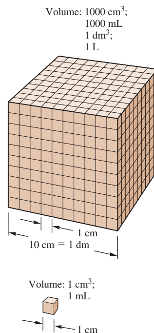
Figure 1.8 The relationships among various volume units.
