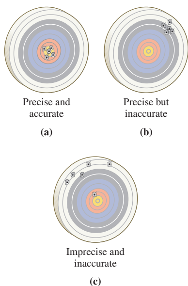
Figure 1.10 An illustration of precision and accuracy in replicate experiments.
