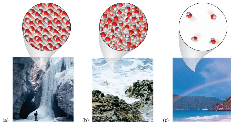
Figure 1.5 The three states of matter exhibited by water: (a) solid, as ice; (b) liquid, as ocean water; (c) gas, as humidity in the air.
