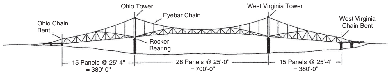
Fig. 2.2 Elevation of Silver Bridge over Ohio River, Point Pleasant, West Virginia (NTSB, 1970).
