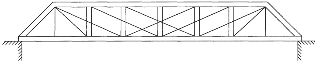
Fig. 1.10 Double-intersection Pratt—credited to Squire Whipple.
