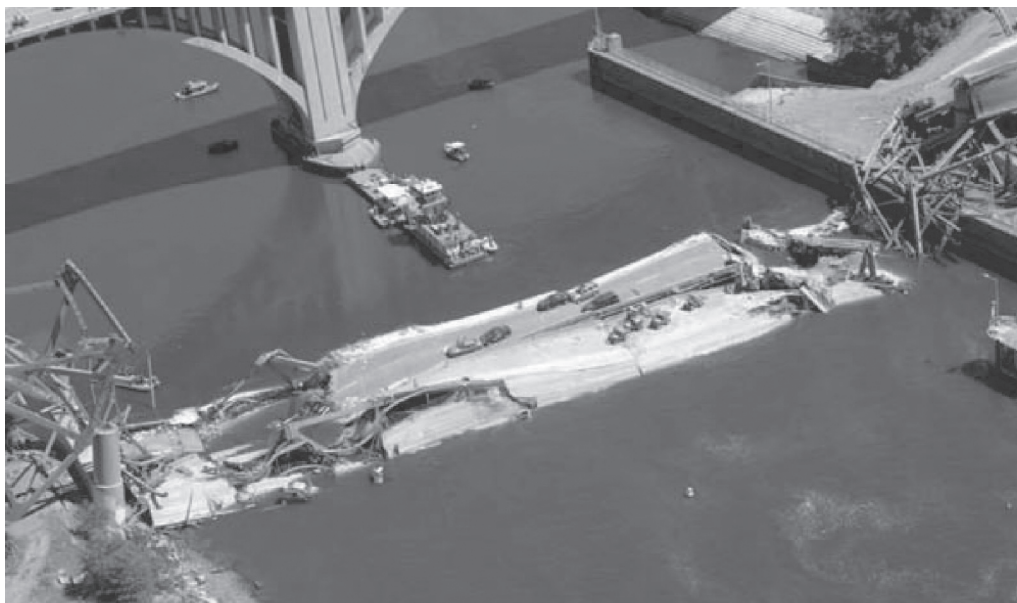
Fig. 2.16 Collapsed bridge center section, looking southeast. (NTSB, 2008).
