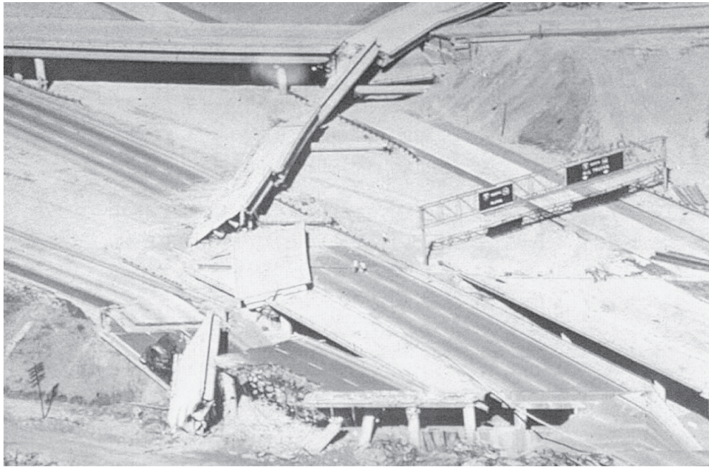
Fig. 2.4 View looking north at the I-5 and I-210 interchange after the quake showing the collapsed South Connector Overcrossing structure (bridge 2) in the center, the North Connector Overcrossing structure (bridge 3) at the top, and bridge group 4 at the bottom. (Photo courtesy E. V. Leyendecker, U.S. Geological Survey.)
