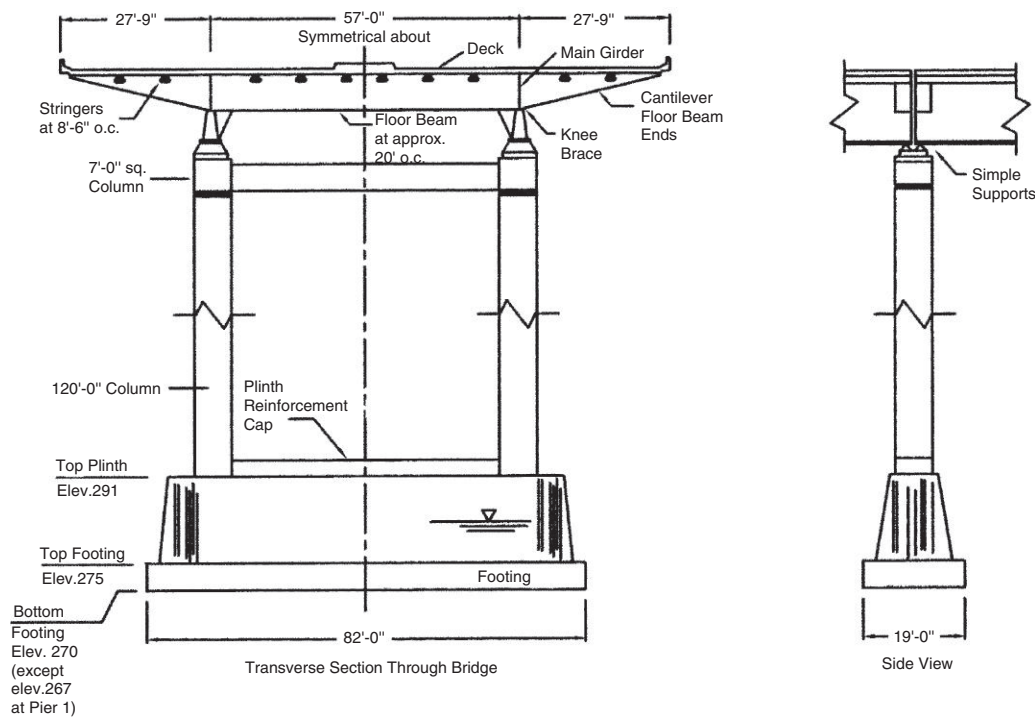
Fig. 2.10 Sections showing the Schoharie Creek Bridge pier supported on a spread footing. (NTSB, 1988).
